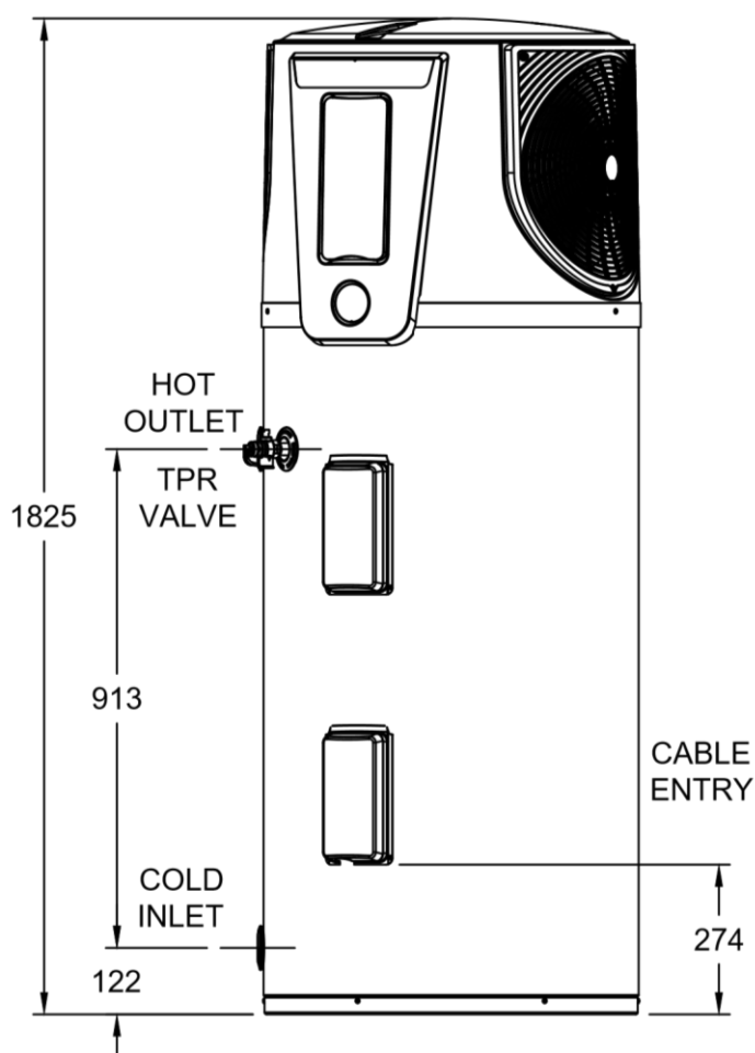
DIMENSIONS 571D270 R513A HEAT PUMP WATER HEATER
